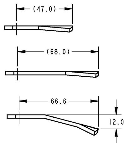
LOCK CAM OPTIONS
